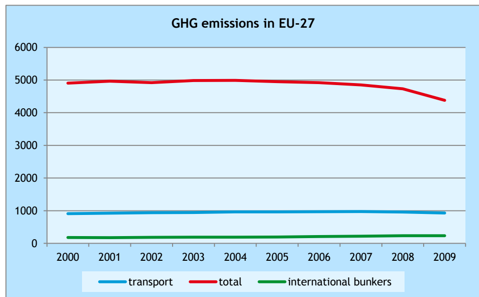
Figure 4 Total and transport GHG emissions in EU-27 (Mtonne per year)
