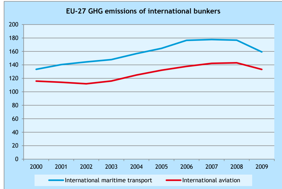
Figure 5 GHG emissions of international bunkers on basis of fuel sales (Mtonne per year)
